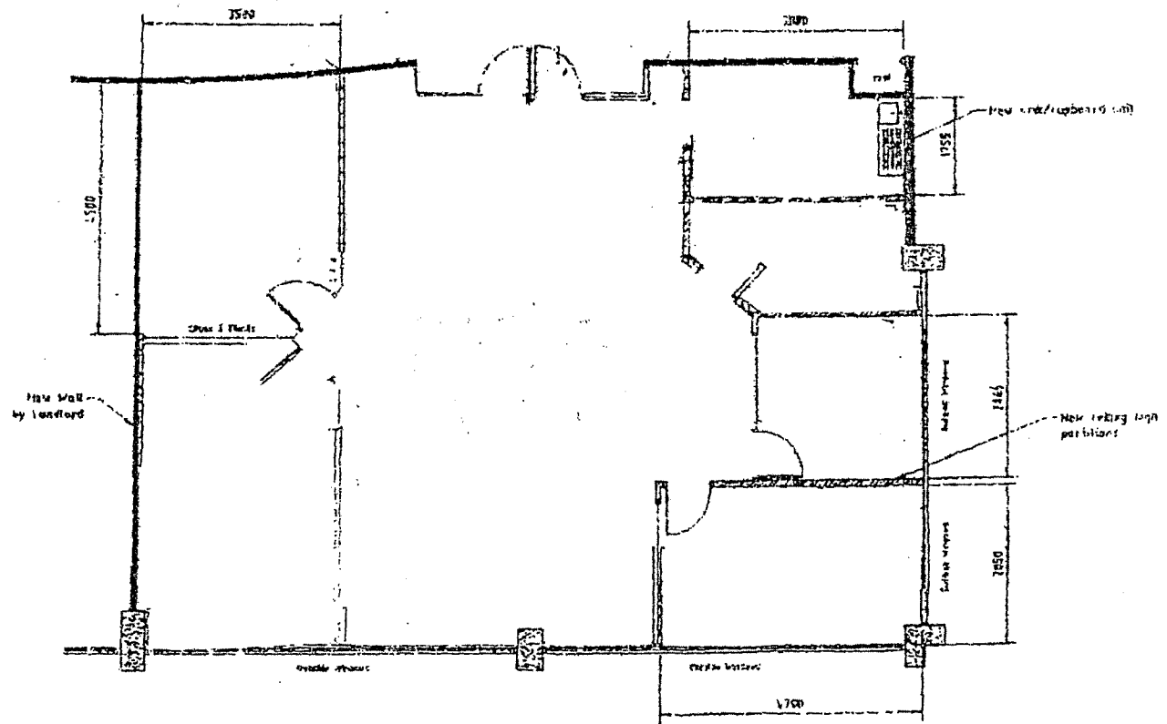
Floor Plan | Floor Area: 140 sqm |
